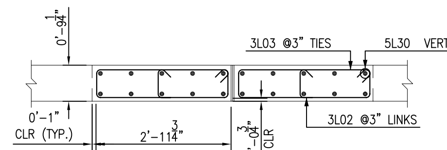
TYPICAL PIER ARRANGEMENT
