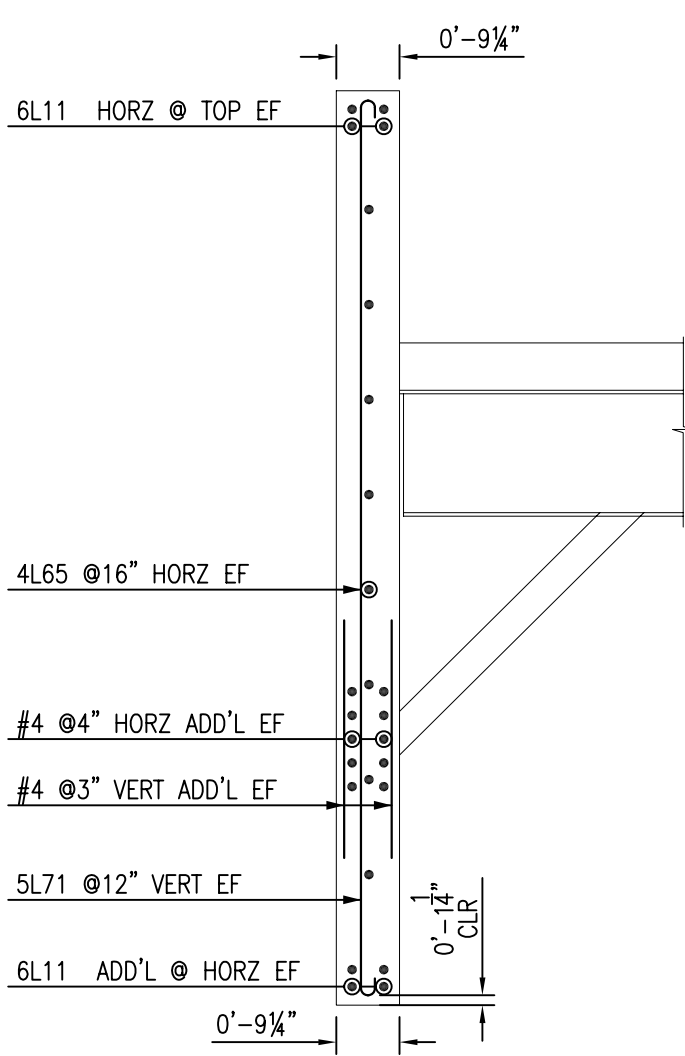
TYPICAL SPANDREL ARRANGEMENT
