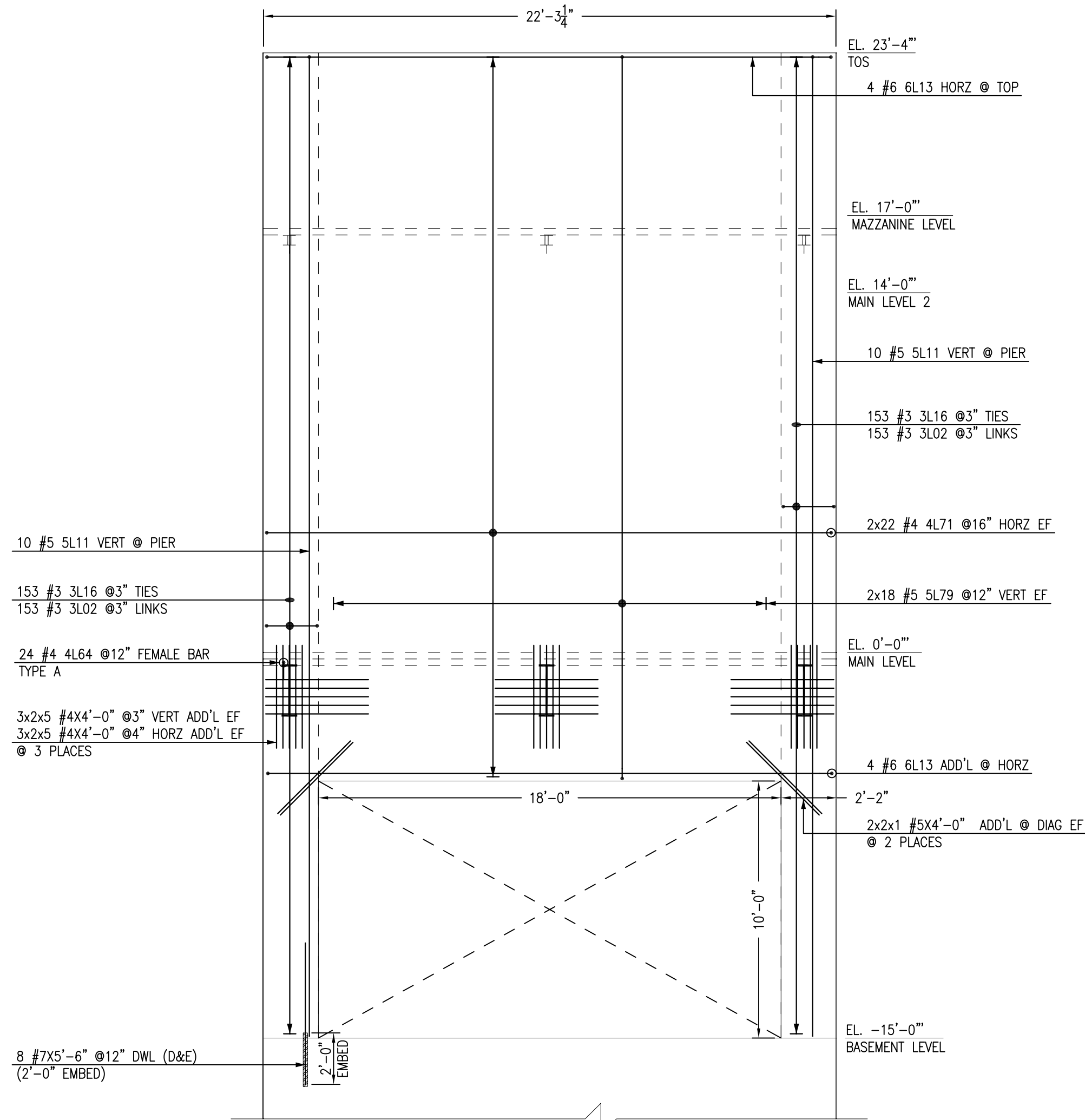
(9/8" THK PANEL) PANEL SCALE - 1/4"=1'-0" REF:1/S3.01
