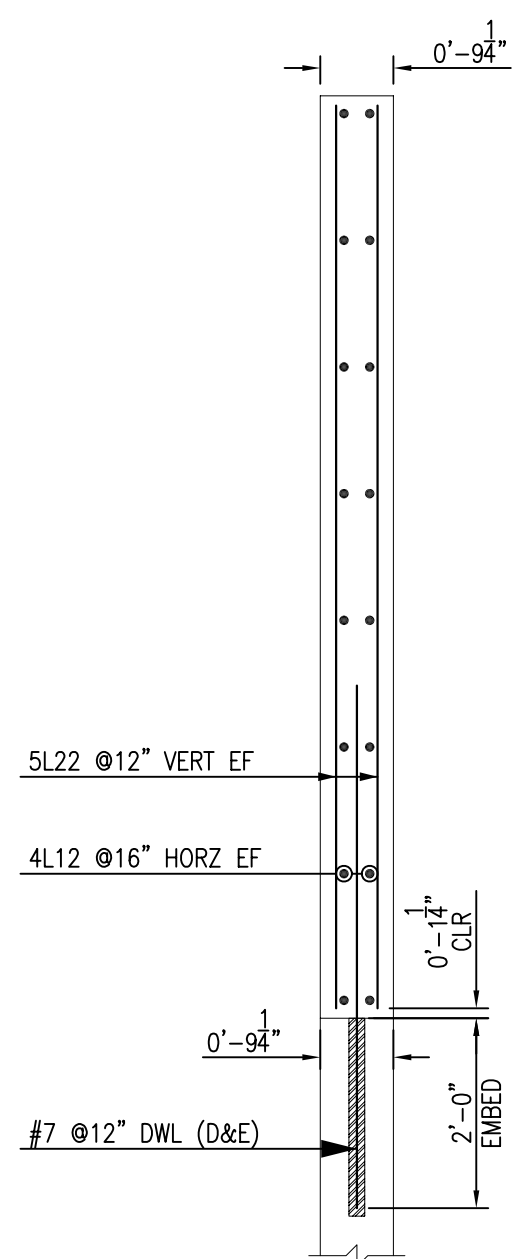
TYPICAL PANEL BAR ARRANGEMENT
