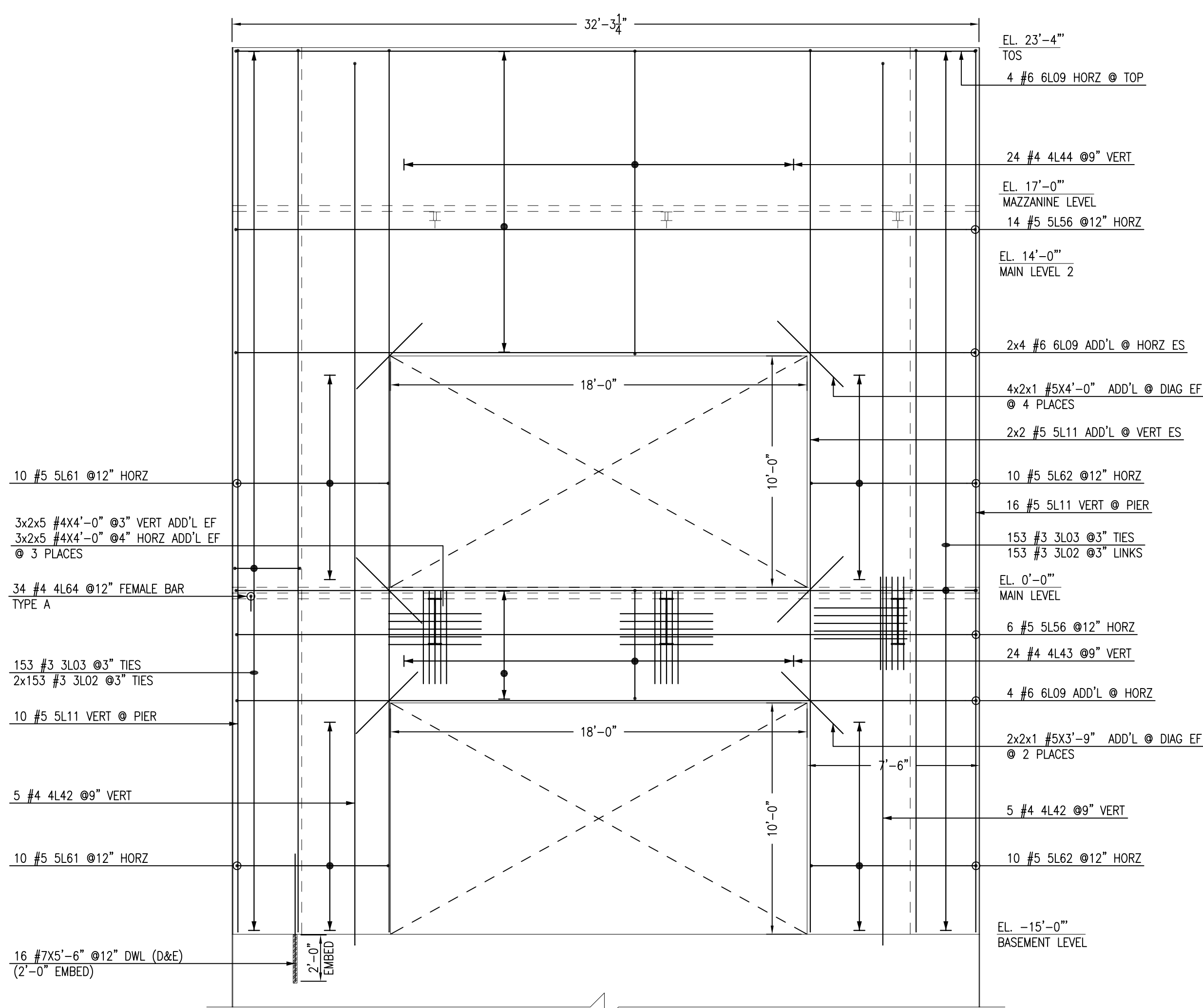
(9/8" THK PANEL) PANEL SCALE - 1/4"=1'-0" REF:1/S3.01
