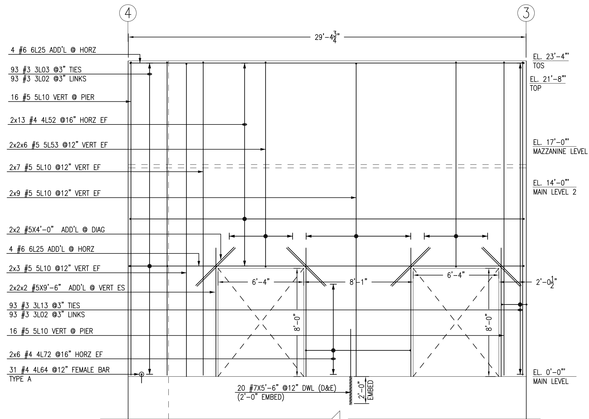
(9/8" THK PANEL) PANEL SCALE - 1/4"=1'-0" REF:1/S3.01
