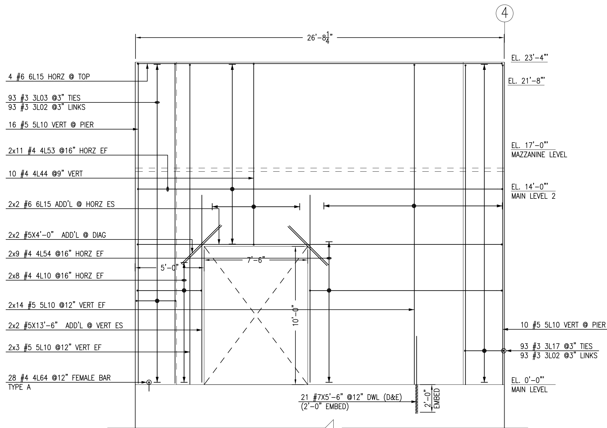
(9/8" THK PANEL) PANEL SCALE - 1/4"=1'-0" REF:1/S3.01
